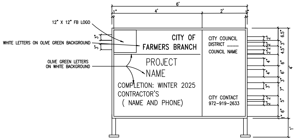
SIGN FRAME DETAIL
