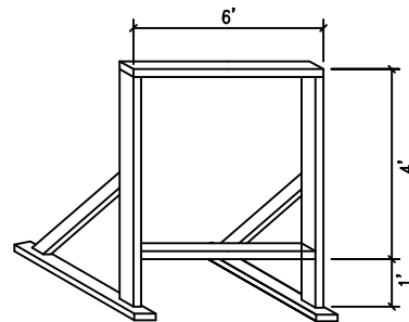
SIGN FRAME DETAIL
