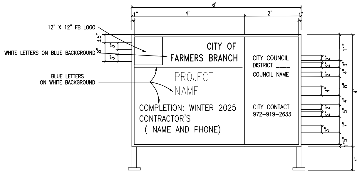
SIGN FRAME DETAIL
