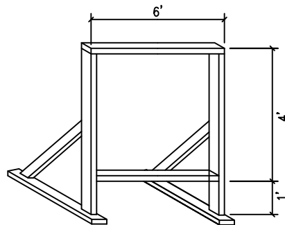
SIGN FRAME DETAIL
