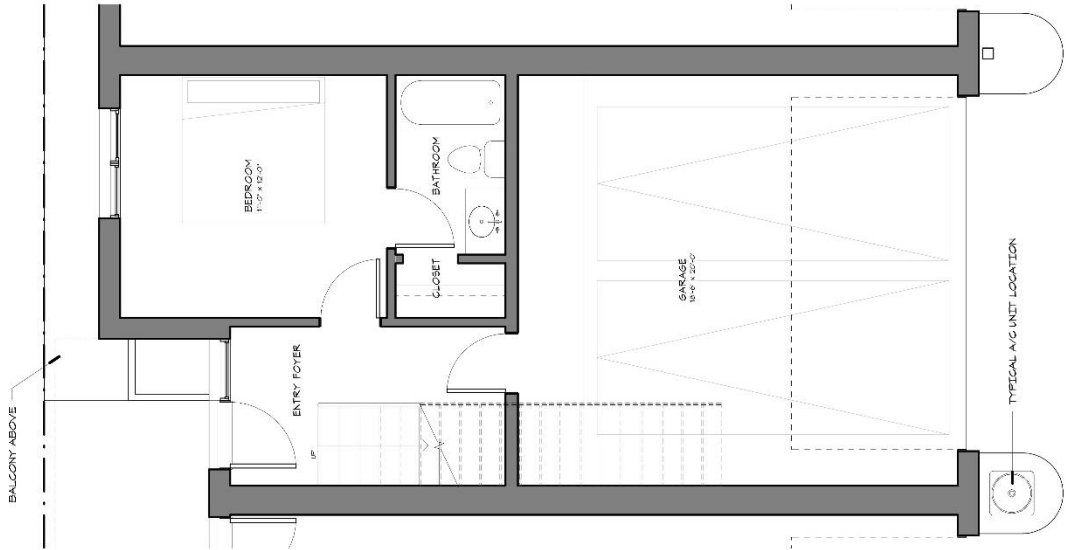
1 FIRST FLOOR 295 SF (A/C) SCALE: 1/4" = 1'-0"
