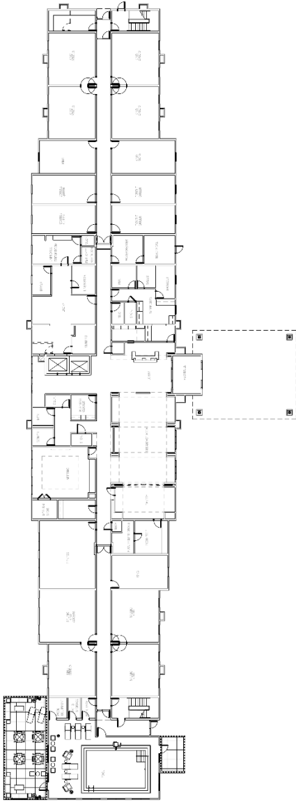
1. GROUND FLOOR PLAN
