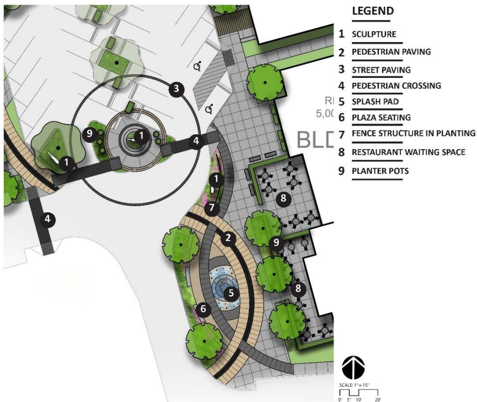
MUSTANG CROSSING: SCHEMATIC DESIGN- OCT 19, 2016
