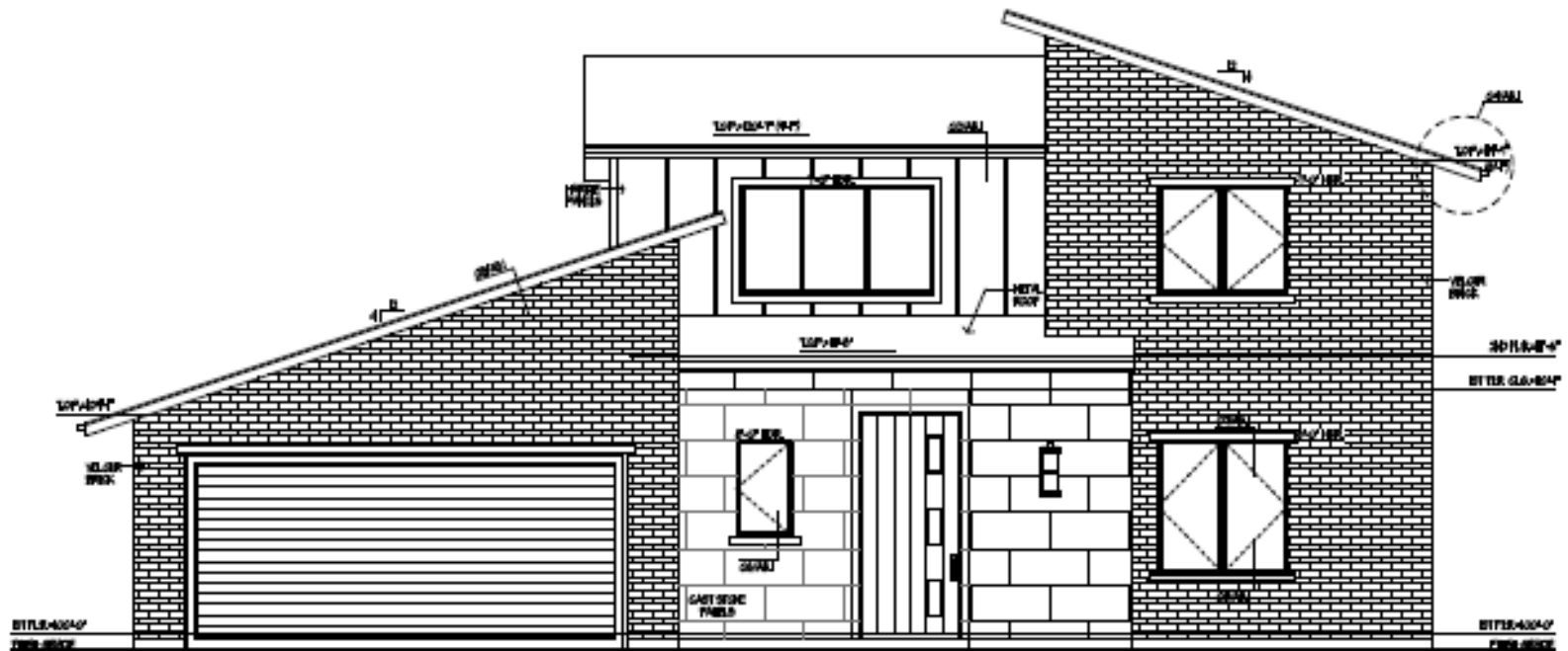
1 FRONT ELEVATION
