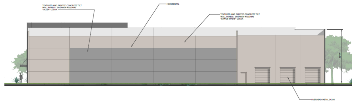
BUILDING A - WEST ELEVATION
