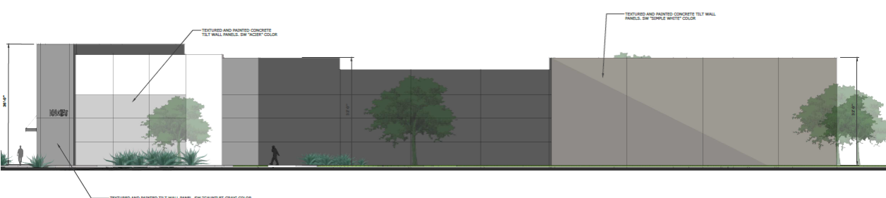
BUILDING B - NORTH ELEVATION
