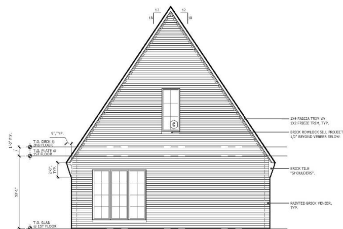
02 REAR ELEVATION - WEST FACE
