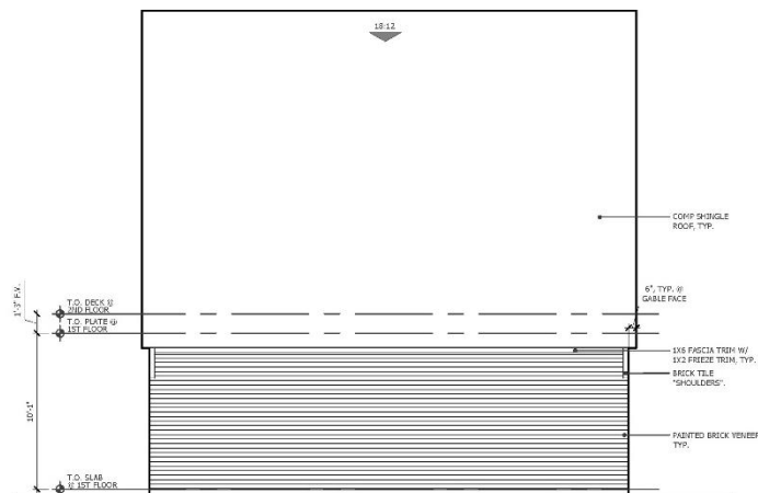
04 SIDE ELEVATION - EAST FACE
