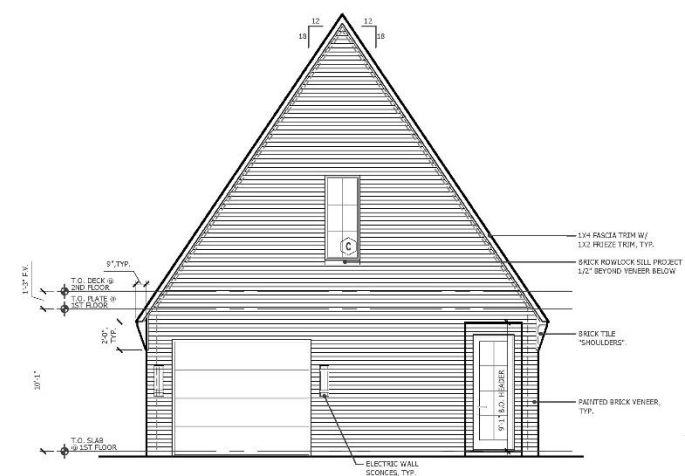
01 FRONT ELEVATION - EAST FACE
