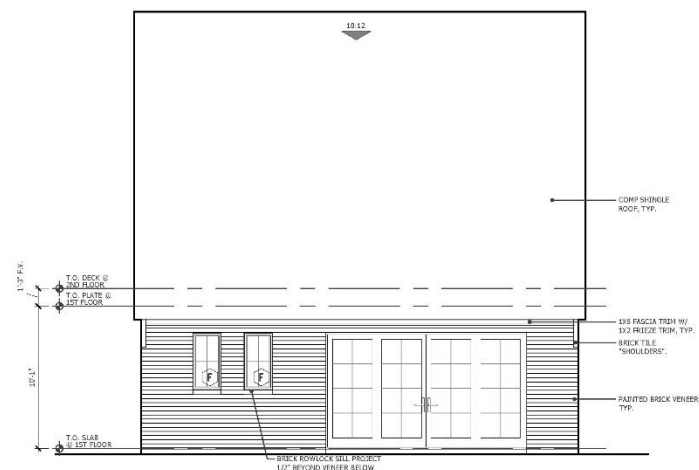
03 SIDE ELEVATION - NORTH FACE
